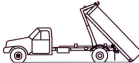
MAX. DUMPING ANGLE 46 DEG
